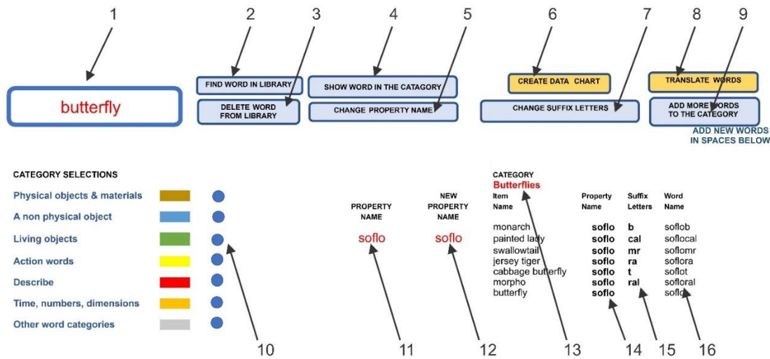
Fig 8 Opening Screen of Computer Program
